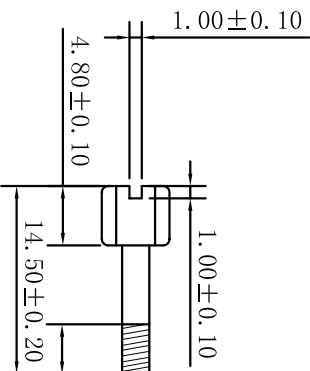
UNC #4-40 Hexscrew
